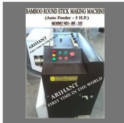
Bamboo Stick Making Machine
